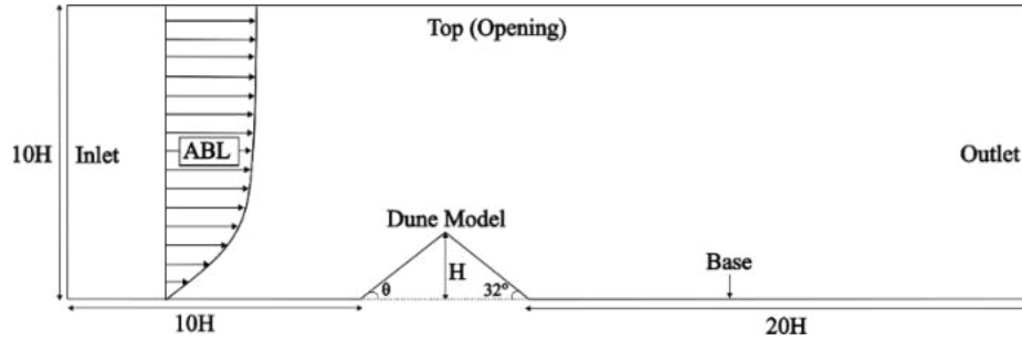
Figure 2. Dimensions of the Computational Domain
