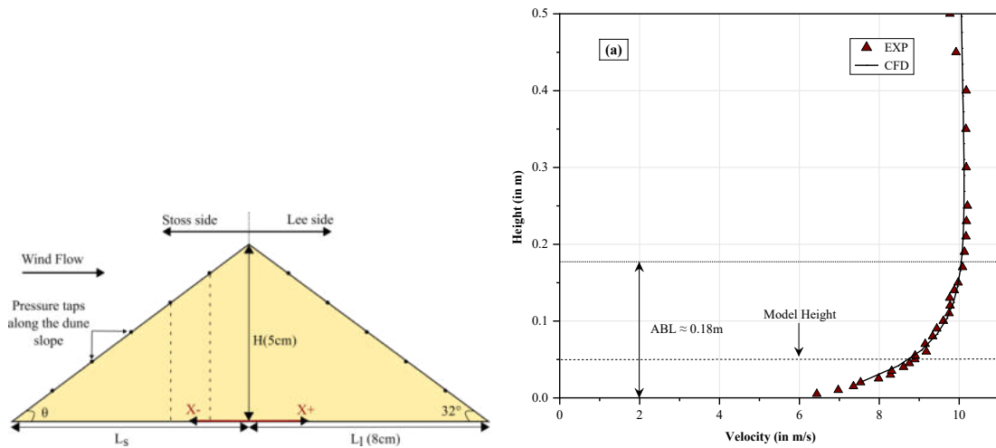
Figure 1. (a) Dune model with varying stoss slope and pressure tap location reference (depicted through X) along base lengths on stoss ( L_s ) and lee side ( L_l ) (b) Inlet wind velocity profile
