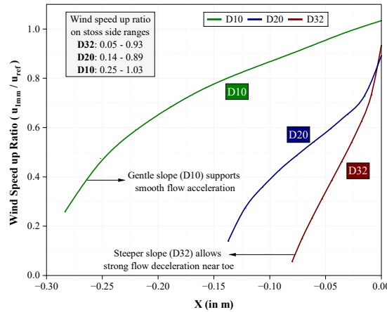
Figure 4. Wind Speed up ratio along the stoss slope of dune
