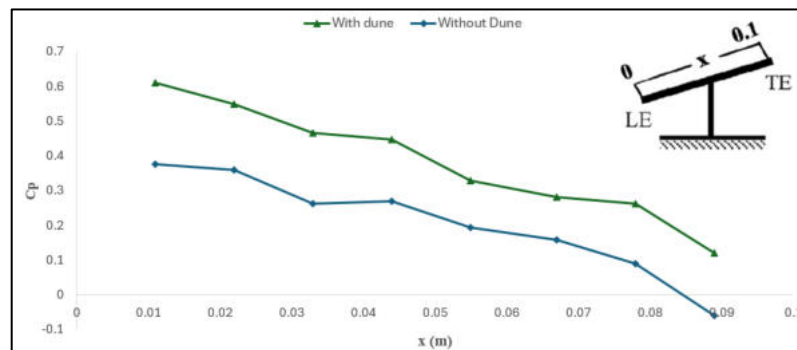
Figure 2: Graph represents the C_p variation for both the configurations
